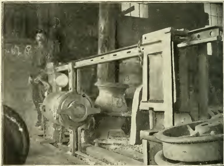
HOME-MADE WHEEL PRESS IN WAUCHUSETT RESERVOIR.
